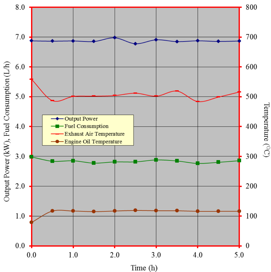
Figure 4. Performance characteristic curves during the continuous running test of the YAMADA PLUS 189F diesel engine
