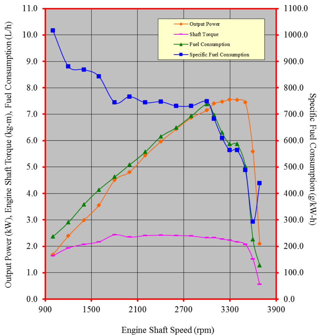
Figure 3. Performance characteristic curves of the YAMADA PLUS 189F diesel engine
